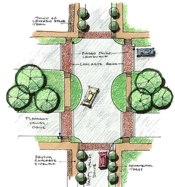
Raised Paver Crosswalks at Pleasant Valley Drive
