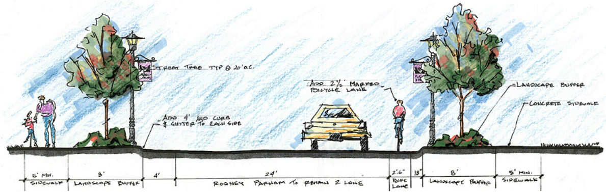
Rodney Parham Street Improvements with Bike Lane/ Landscape Buffer and Sidewalks
