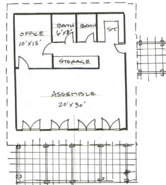
Community Center Floor Plan
